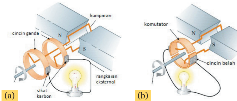
Gambar 6.32 (a) Generator AC, (b) Generator DC
