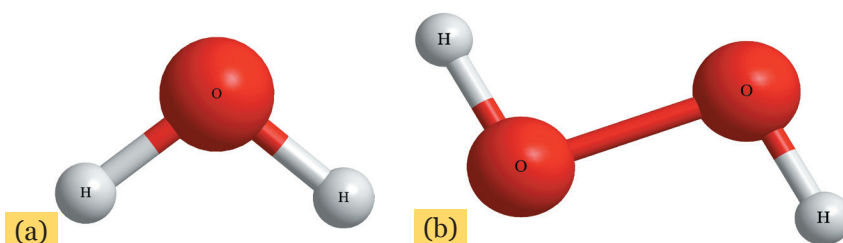
Gambar 8.5 Molekul (a) H_2O , (b) H_2O_2
