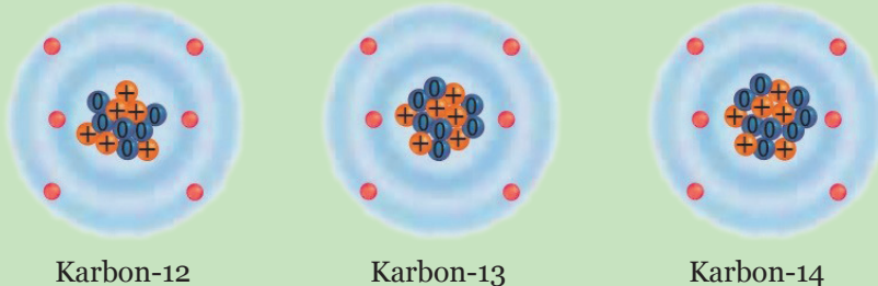
Gambar 8.14 Isotop-isotop Atom Karbon
